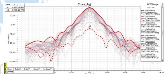
Fig. 11 Cross-polarization plot on Gain in LHCP and RHCP vs theta.
