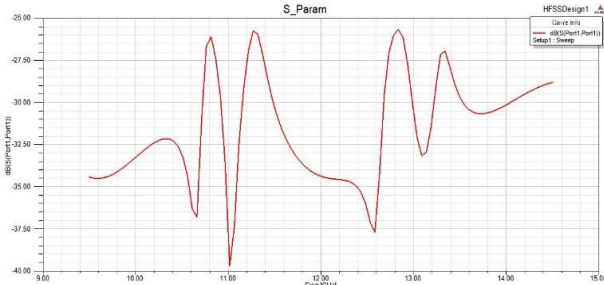
Fig. 7 Horn antenna return loss
