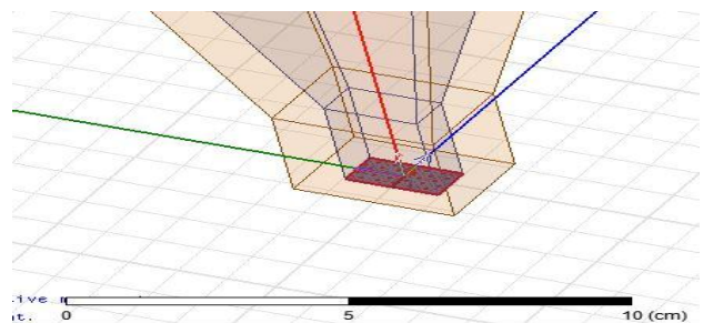
Fig. 6 Horn antenna excitation for feed on HFSS
