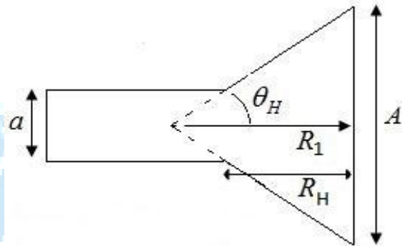
Fig. 2 Broadside dimensions.
