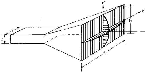
Fig. 1 The standard pyramidal horn antenna
