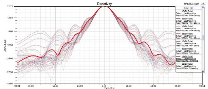
Fig. 12 Directivity vs theta.
