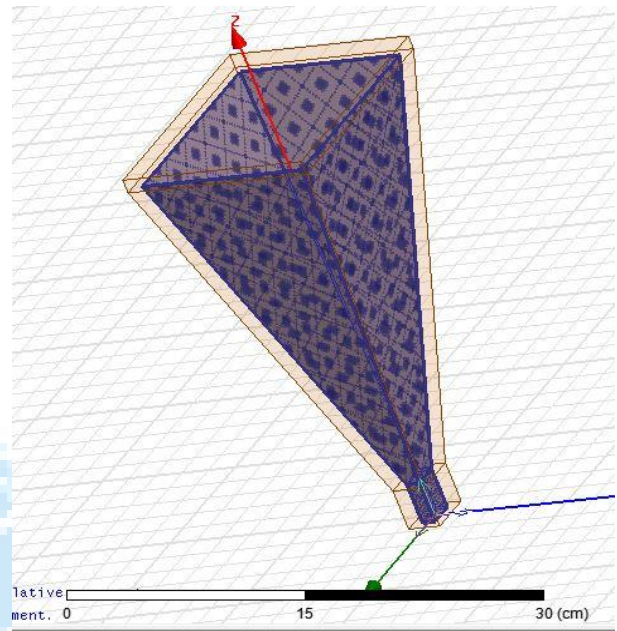
Fig. 4 Horn antenna implementation on HFSS
