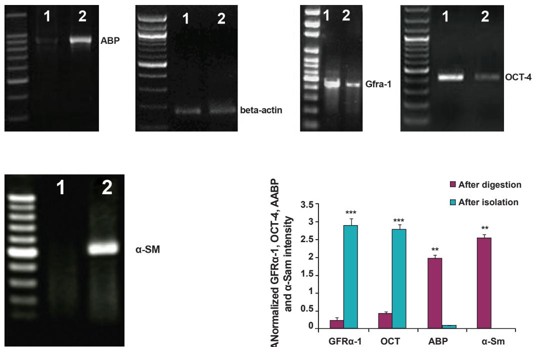
Fig 1: Expression analysis of premeiotic and somatic testicular marker genes GFR \alpha -1, OCT4, ABP and \alpha -Sm.1, after MACS isolation 2, after second digestion. \beta -actin was used as an internal control. Densitometric analysis is shown in the histogram.
