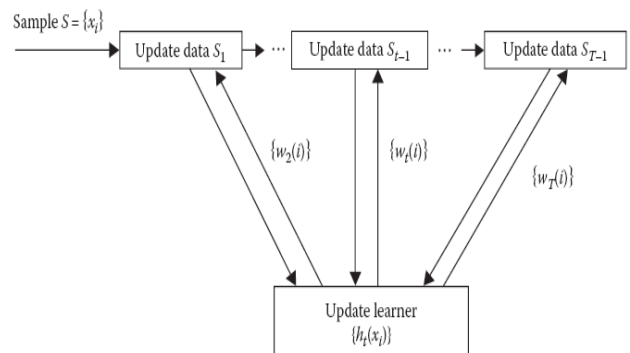
Fig. 5- Workflow of Adaboost
