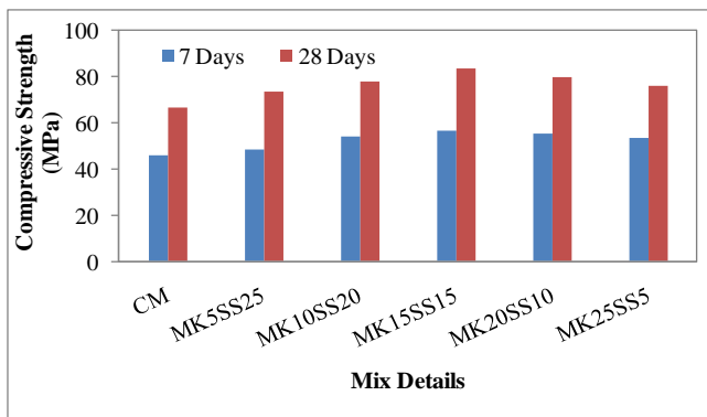
Fig. 5 Compressive strength test results of various concrete mixes
