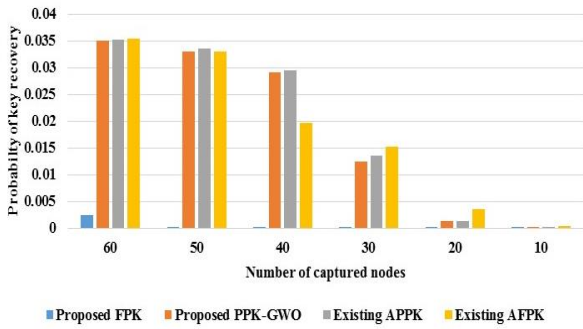
Figure. 3 Comparative examination of diverse scheme on the possibility of key recovery for dissimilar values of i = 10
