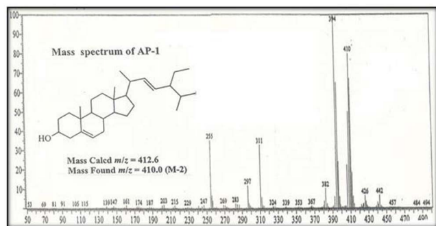
Figure 5. Mass spectrum of isolated endophytic compound AP-1.
