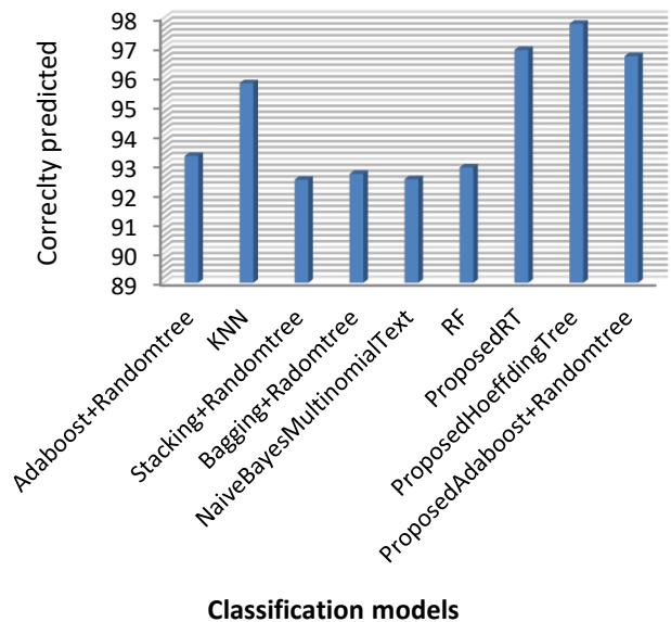
Figure. 7 Performance comparison of proposed classification models to the existing approaches on e-commerce dataset using true positivity and false negativity
