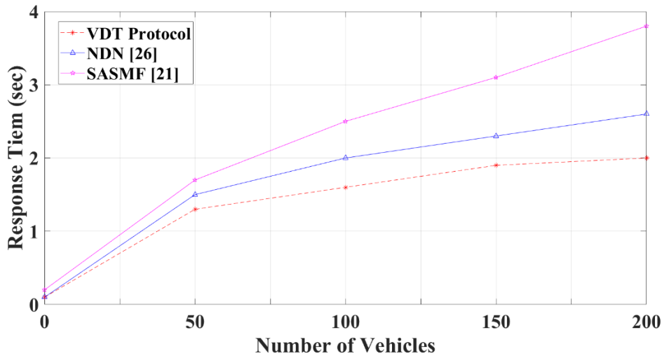
Figure.10 Response time comparison
