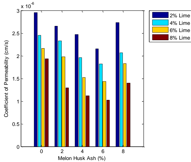
Figure 6: Variation of 28 day permeability with melon husk ash and lime content
