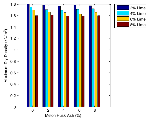
Figure 1: Variation of maximum dry density with melon husk ash and lime content
