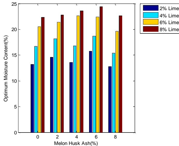
Figure 2: Variation of optimum moisture content with melon husk ash and lime content
