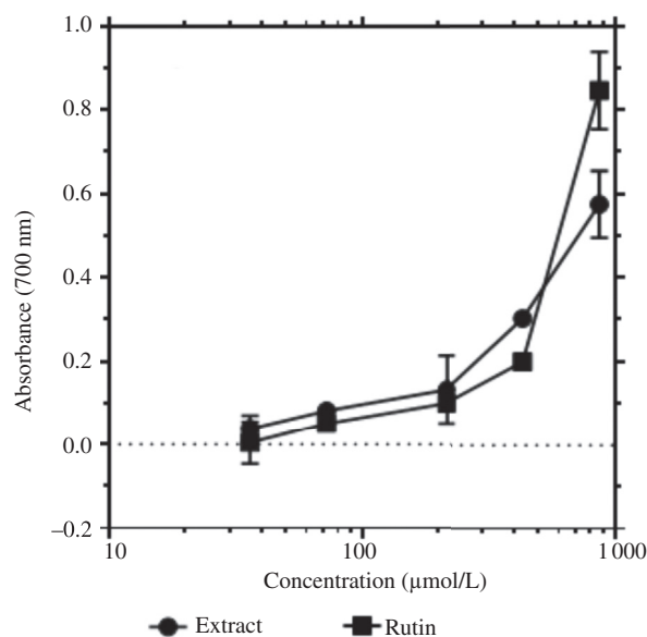
Figure 3. Reducing power of ethanolic extract of E. superbum seeds and rutin based on measurement of Fe 3+ –Fe 2+ transformation. Data are expressed as mean ± SEM (n = 4).
