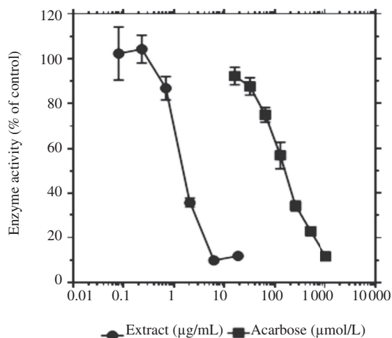
Figure 4. Anti- \alpha -glucosidase activity of the crude methanolic extracts of E. superbum seeds and acarbose. Data are expressed as mean \pm SEM ( n = 4 ).
