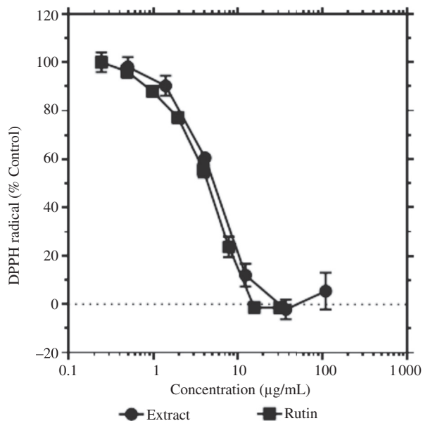
Figure 1. Antioxidant activity of the methanolic extracts of E. superbum seeds and rutin. Data are mean ± SEM values (n = 4).
