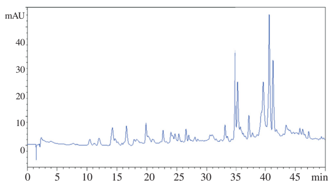
Figure 2. HPLC profile of the crude extract of E. superbum seeds.
