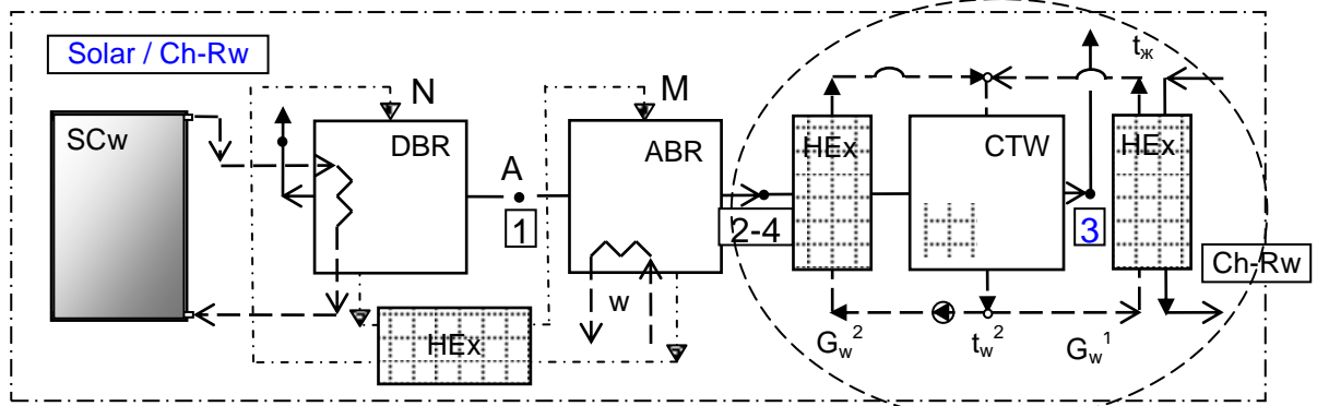
Figure 7 – Performance analysis of the Ch-Rw ( l = G_a/G_{w\Sigma} = 1.0 and l^* = G_w^1/G_w^2 = 1.0 )
