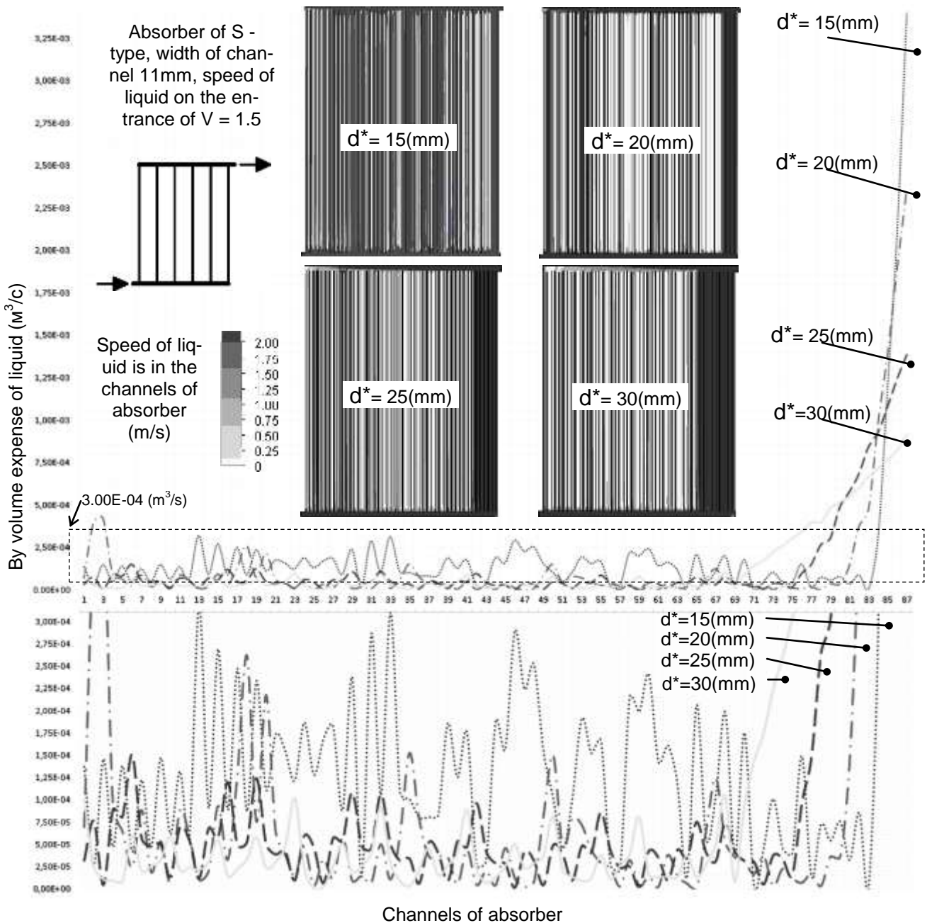
Figure 5 – Distribution of liquid in channels at V=1.5 (m/s) on an entrance in S-type absorber; the internal ( d^* ) diameter of hydraulic collectors was varied in calculations
