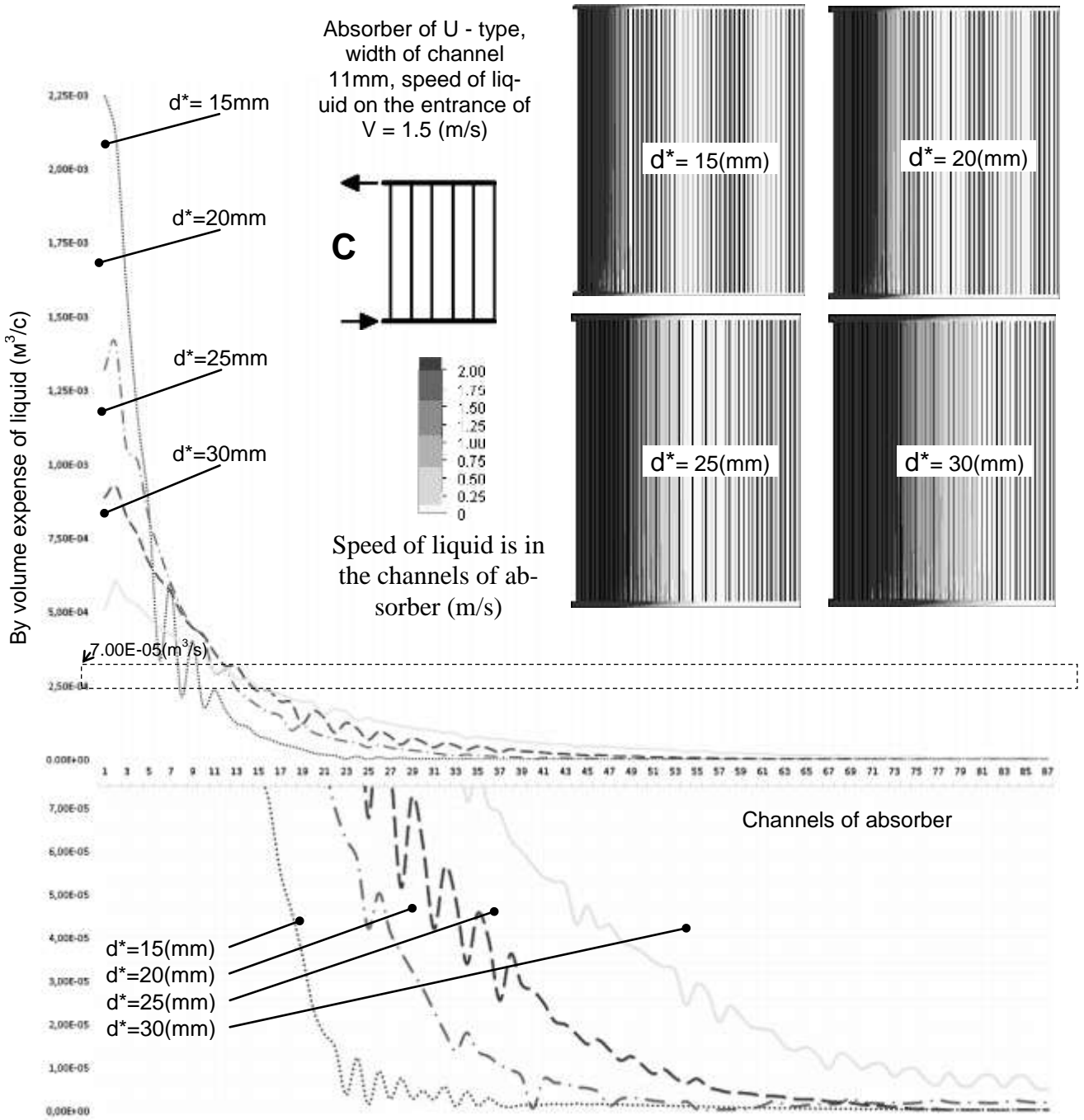
Figure 4 – Distribution of liquid in channels at V=1.5 (m/s) on an entrance in U-type absorber; the internal ( d^* ) diameter of hydraulic collectors was varied in calculations
