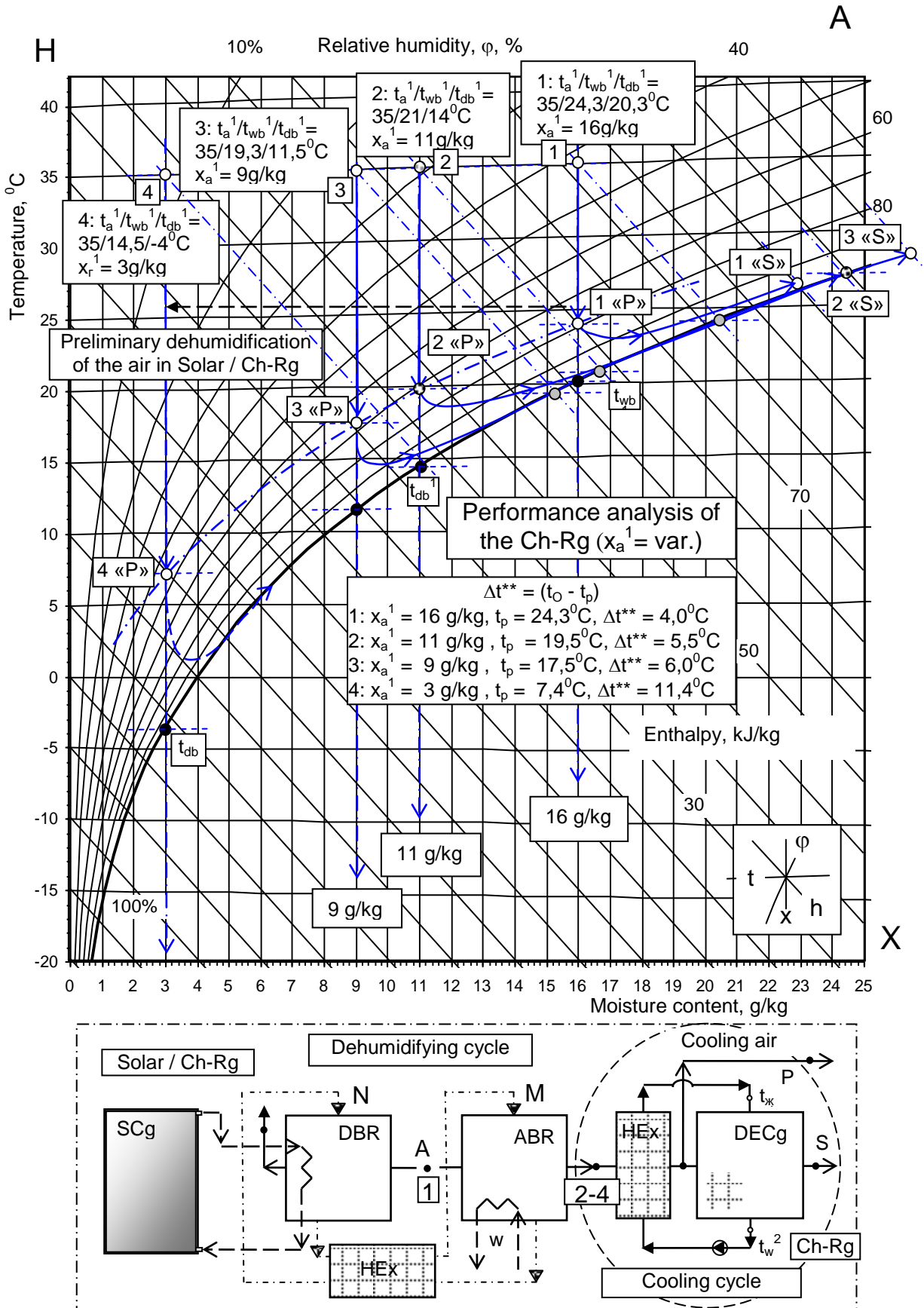
Figure 6 – Performance analysis of the Ch-Rg ( l = G_p/G_s = 1.0 ).
