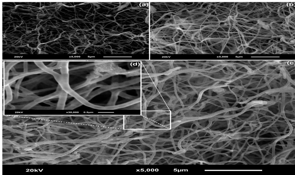
Figure 4: SEM micrograph of fibers of SiO 2 -HA at 5,000x after 800°C heat treatment and SiO 2 flow of (a) 1.2 mL/h, (b) 0.8 mL/h and (c) 0.4 mL/h before the heat treatment. Constriction along the fibers is shown in figure 4(d).
