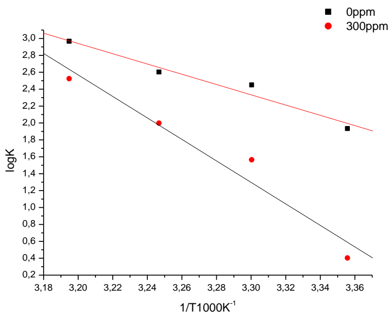
Fig.4. Plot of \log(k) versus 1/T \times 10^3, K^{-1} for carbon steel in decanted water Solution in absence and in presence of 300ppm of inhibitor.
