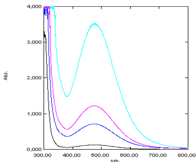
Fig.6. UV-spectra of the solutions containing different concentration of acetylsalicylic acid after 3h immersion of carbon steel.
