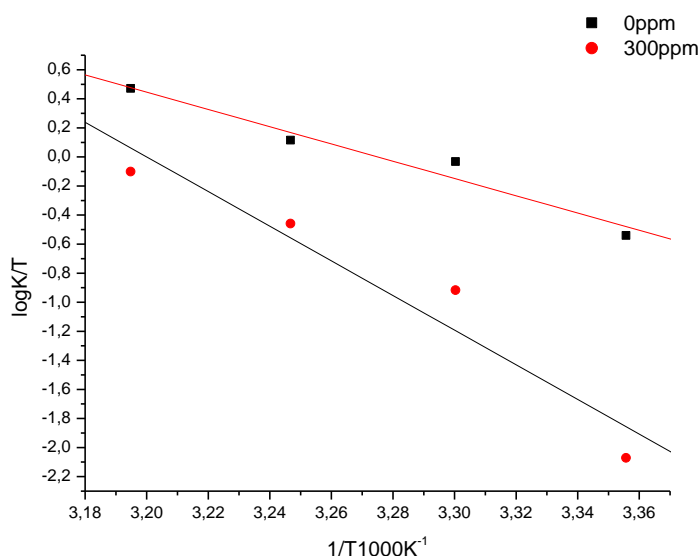
Fig.5. Plot of \log(\text{corrosion rate}/T) versus 1/T \times 10^3, \text{ K}^{-1} for carbon steel in decanted water Solution in absence and in presence of 300 ppm of inhibitor.
