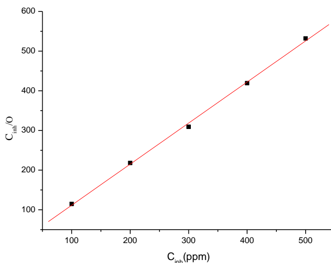
Fig.3. Plot of C_{inh}/\Theta versus C_{inh} for carbon steel in decanted water solution in presence of different concentrations of inhibitor
