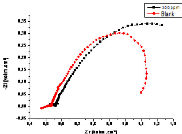
Fig.8. EIS of carbon steel in decanted water in absence and presence of 300ppm
