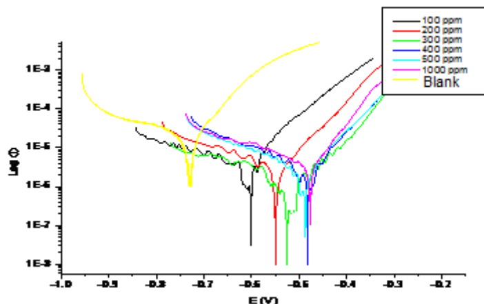
Fig 2: Polarization curves of carbon steel in decanted water in the absence and various concentrations of inhibitor
