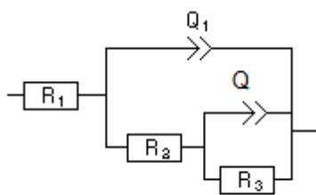
Fig.9. Equivalent circuit used to fit the EIS.
