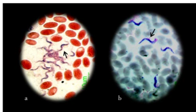
Figure 1. Microscopical examination of the stained blood smear from a naturally infected camel (arrow) (1 000 \times ).
