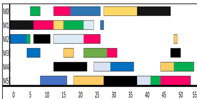
Figure 5: Gant chart for instance FT06 on CP-2
