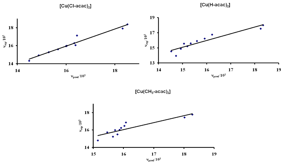
Fig. 3: The plots of the observed v_{max} values against the calculated v_{max} values for complexes.
