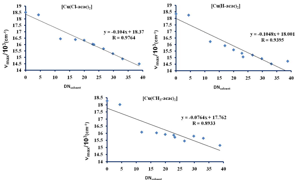
Fig. 2: Dependence of the v_{max} values of complexes on the solvent DN values.
