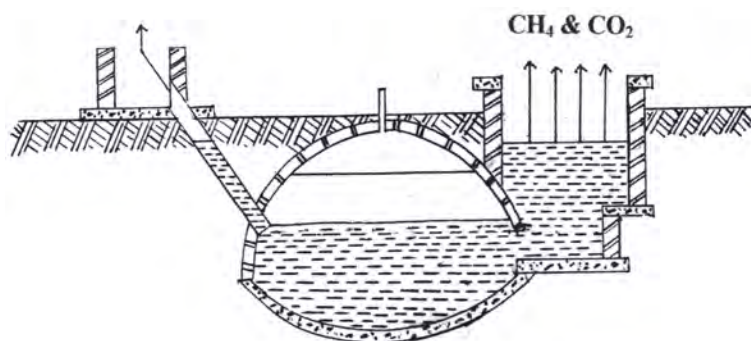
Fig. 1: CH 4 and CO 2 emission from conventional biogas plant
