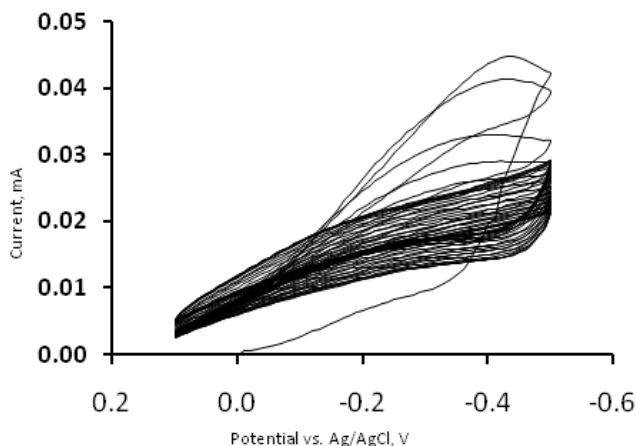
Fig. 1 Cyclic voltammograms for deposition of platinum nanoparticles on carbon fiber
