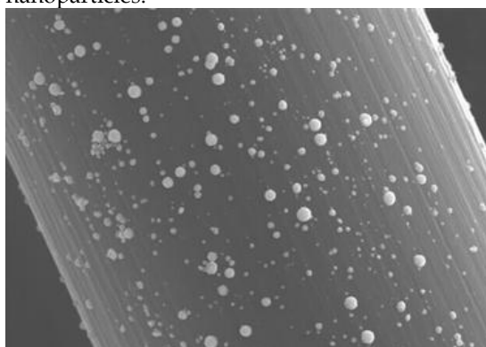
Fig. 2 SEM micrographs of platinum nanoparticles deposited on carbon fiber by cyclic voltammetry
