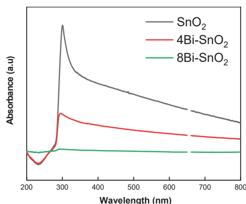
Fig. 4. UV-Vis spectra of Bi 3+ -SnO 2 nanocomposite with Bi 3+ mass ratios of 0% (grey), 4% (red), and 8% (green).
