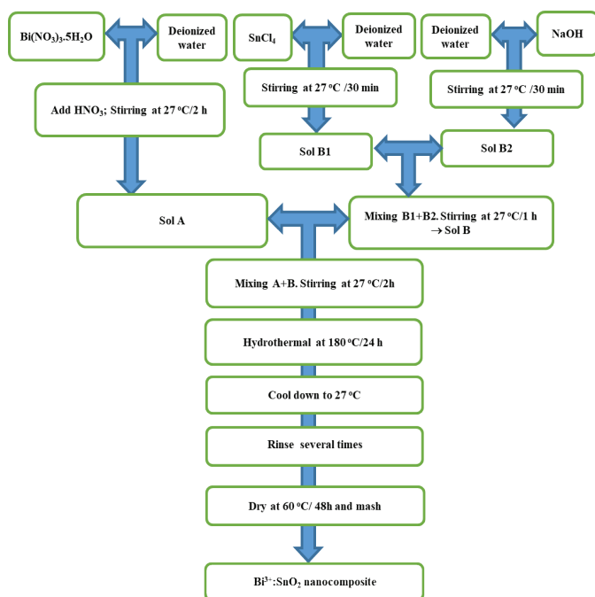
Fig. 1. Diagram of Bi 3+ -doped SnO 2 nanocomposite synthesis.
