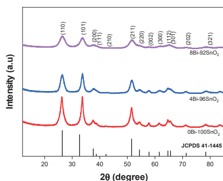
Fig. 2. XRD patterns of Bi 3+ -doped SnO 2 nanocomposites with different Bi 3+ mass ratios (0, 4, 8 wt%). Diffraction peak positions of SnO 2 are taken from JCPDS Card No.41-1445.
