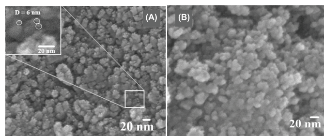
Fig. 3. SEM images of (A) pure SnO 2 and (B) 4Bi-96SnO 2 . The inset shows a small area in the large-scale image.
