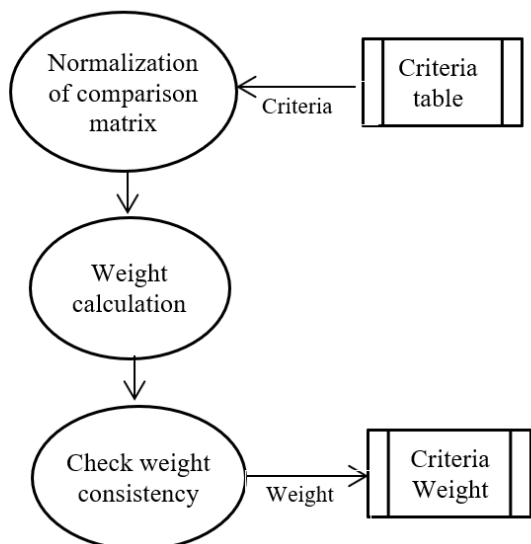
Figure. 4 DFD Level 2 AHP weighting process
