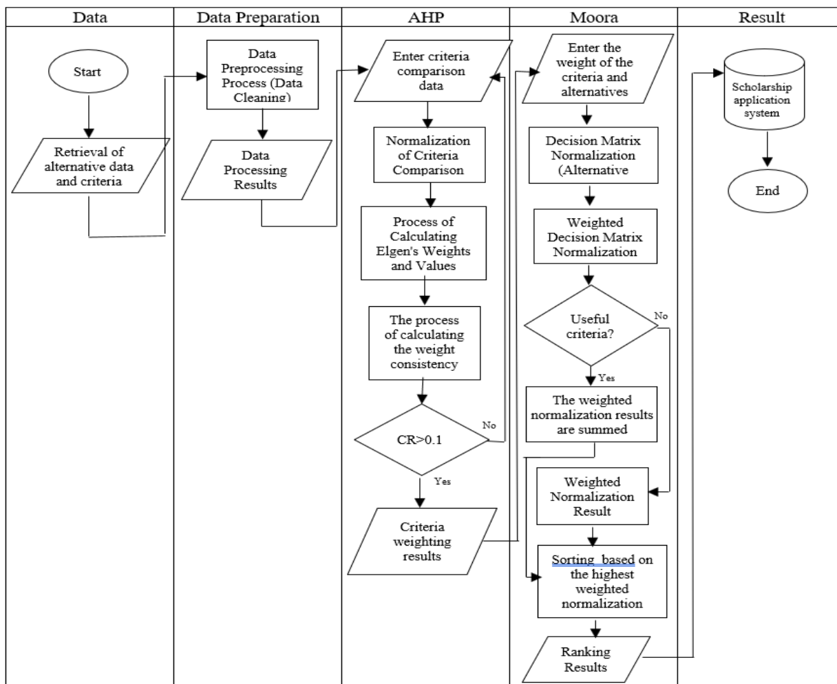
Figure. 6 Flowchart of the application system built
