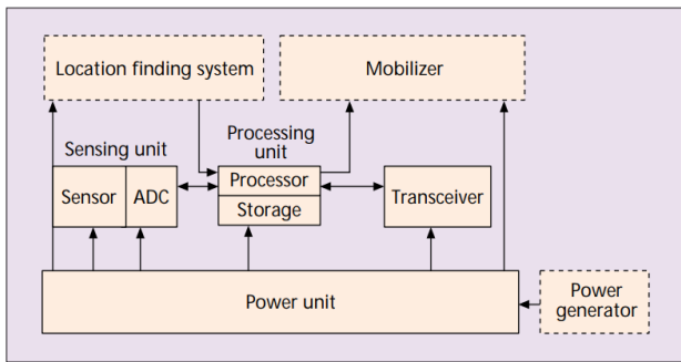
Figure 2. Hardware components of a sensor node
