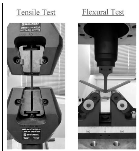
Figure 3. Image of during tensile and flexural test.
