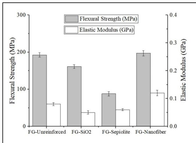
Figure 9. Data extracted from flexural stress curves of unreinforced and reinforced FG composites.
