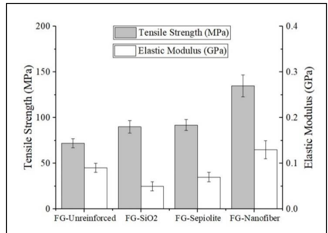
Figure 7. Data extracted from stress-strain curves of unreinforced and reinforced FG composites.
