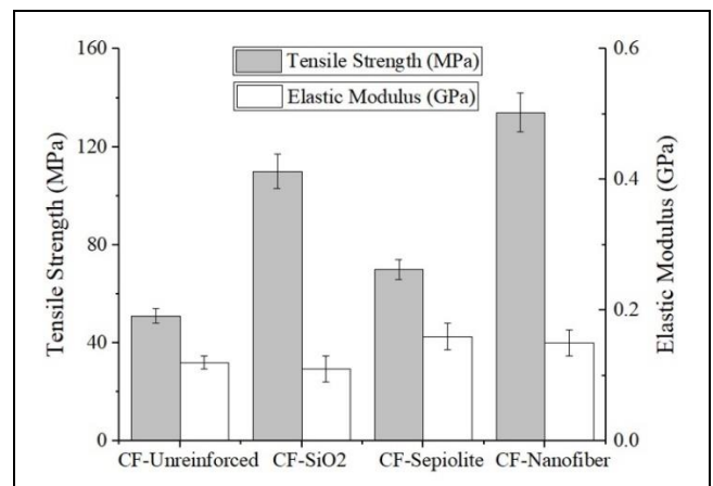
Figure 8. Data extracted from stress-strain curves of unreinforced and reinforced CF composites.
