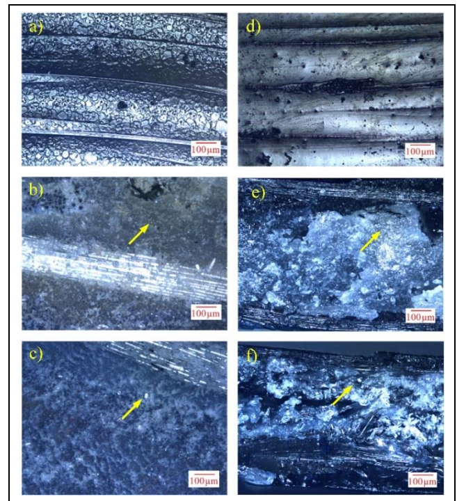
Figure 4. Optic microscope images of unreinforced and reinforced FG and CF composites (100x); a) surface of fiber glass plain. (b): Cross-section of sepiolite reinforced fiber glass composite. (c): cross-section of SiO 2 reinforced fiber glass composite. (d): surface of carbon fiber plain. (e): Cross-section of sepiolite reinforced carbon fiber composite. (f): Cross-section of SiO 2 doped carbon fiber composite.
