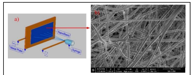
Figure 2(a): Electrospinning technique. (b): The SEM image of PU nanofibers at magnification of 10 000x.
