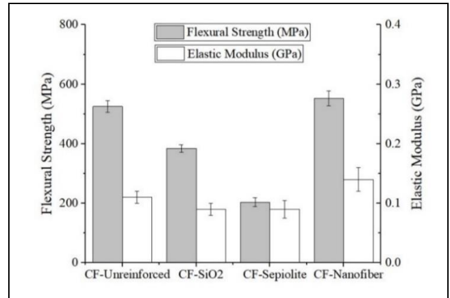
Figure 10. Data extracted from flexural stress curves of unreinforced and reinforced CF composites.
