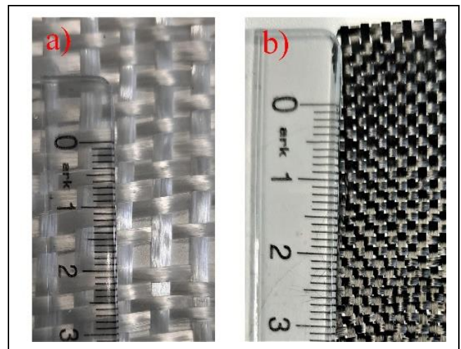
Figure 1. Macro image of fiberglass fabric. (a): and carbon fiber. (b): Plain.
