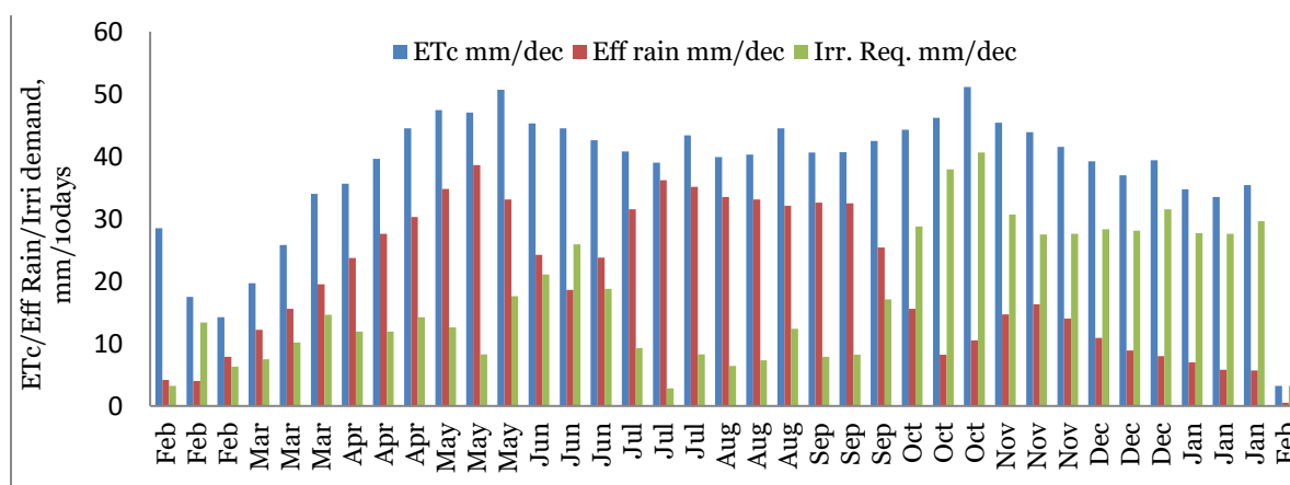
Fig. 2. Monthly crop water and irrigation demand.
