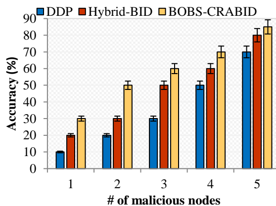
Figure. 14 Accuracy vs. no. of malicious nodes
