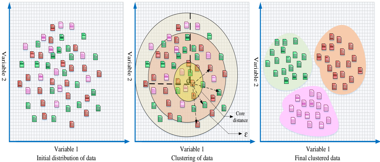
Figure. 4 Optics based clustering
