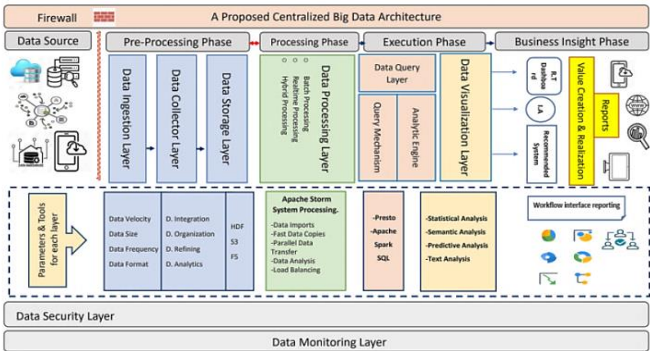
Figure. 1 Architecture of centralized bigdata
