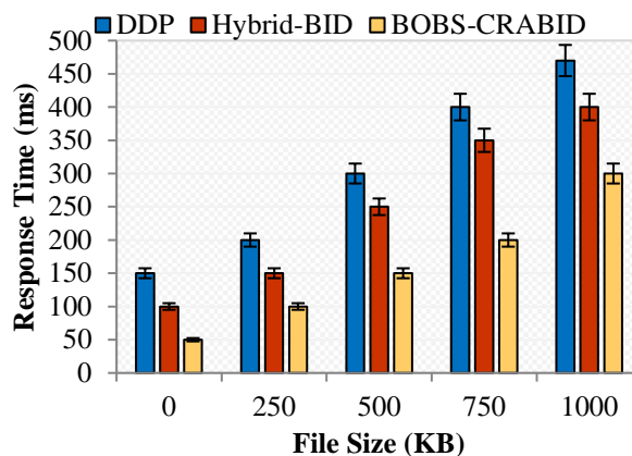
Figure. 11 Response time vs. file size
