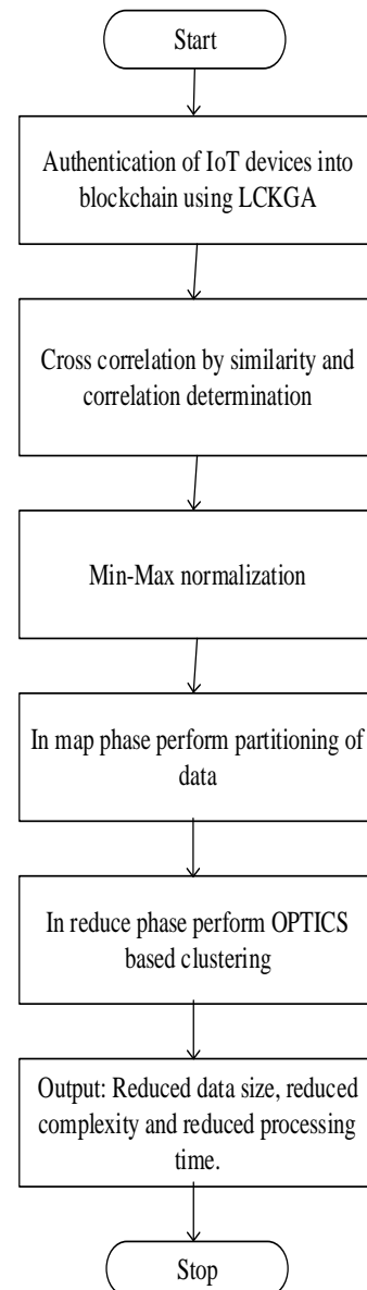
Figure. 5 BOBS-CRABID Flowchart
