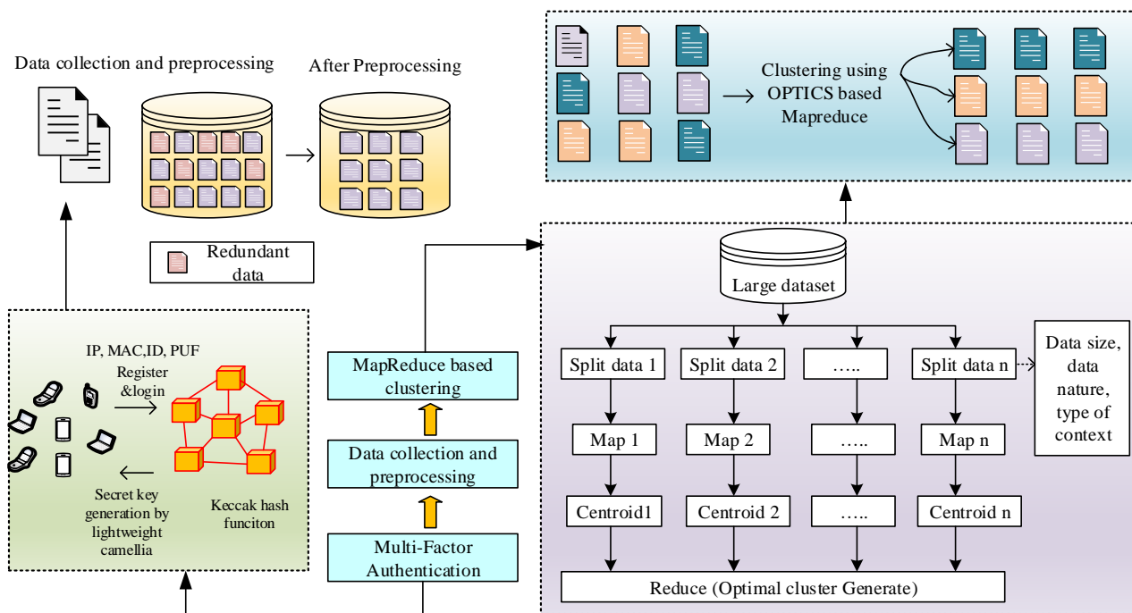
Figure. 2 System architecture
