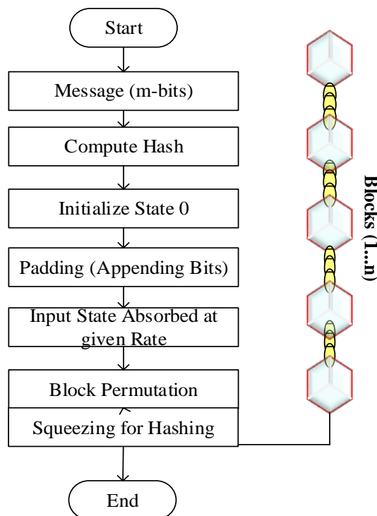
Figure. 3 Keccak hashing
