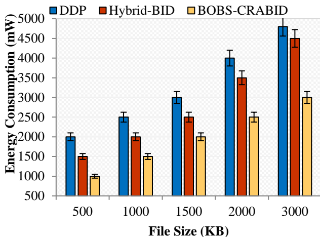
Figure. 12 Energy consumption vs. file size
