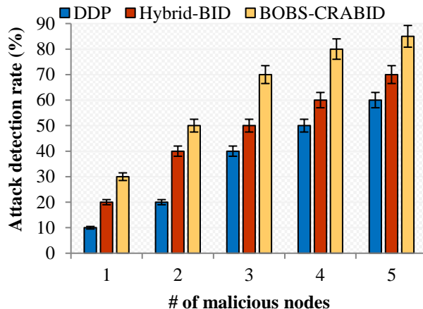
Figure. 13 Attack detection rate vs. no. of malicious nodes
