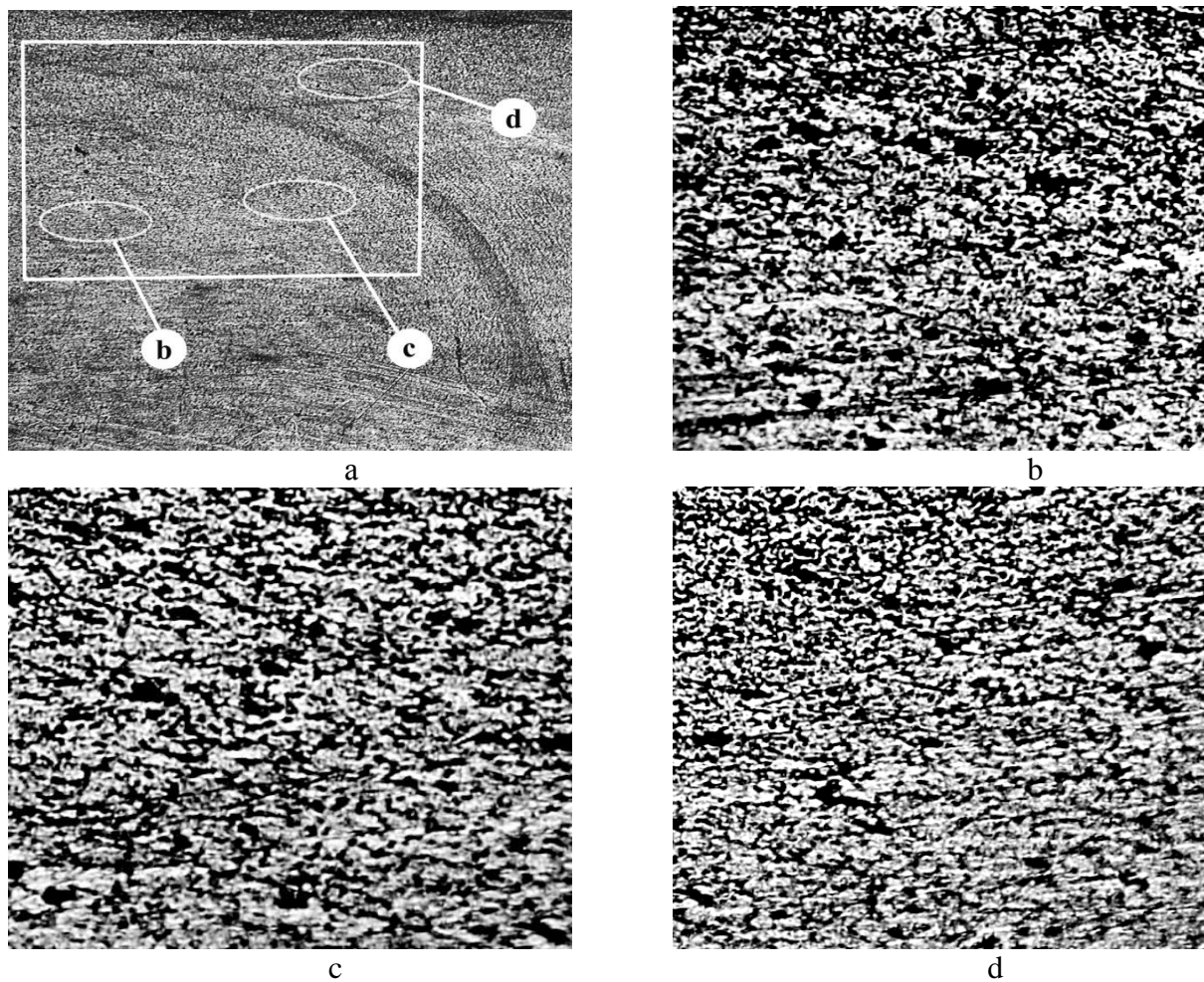
Fig. 3. General view of the area intensive mixing after FSW ( v = 1250 \text{ min}^{-1} ) (a) and enlarged image of the selected fragment depending on heating temperature: (b) -330, (c) -345 and (d) -360°C. Magnification: a - 100; b-d - 350
