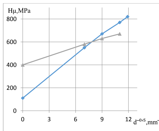
Fig. 4. Influence of the size of grain \alpha - solid solution on microhardness, depending on the temperature of the microvolumes alloy at FSW (▲ - 330, ◆ - 360°C)
