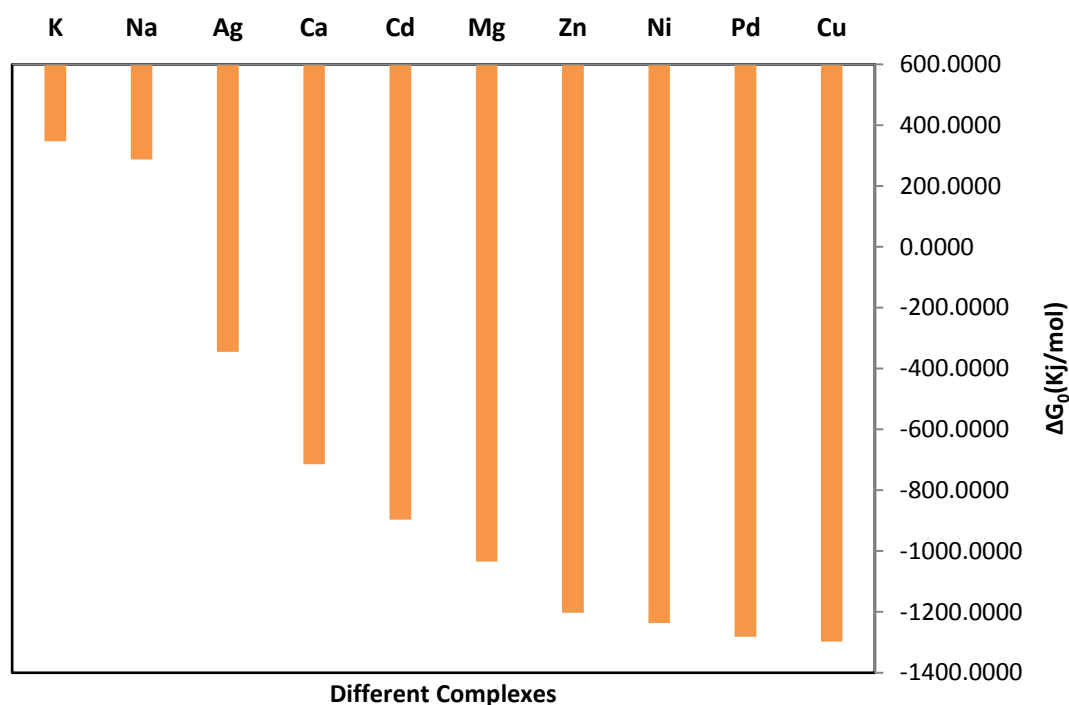
Fig 5. Gibbs free energy changes and of the complexation process in the ambient temperature and gaseous phase.
