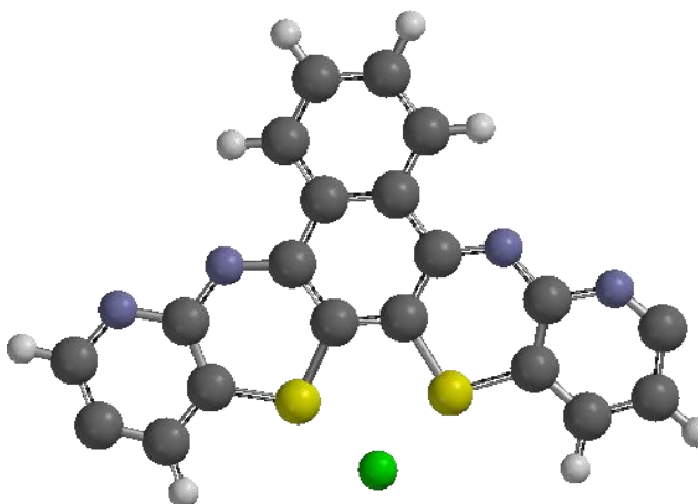
Fig 3. Mode B: Cu 2+ attaches to the ligand via the sulfur atoms.
