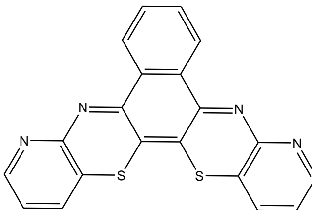
Fig 1. The structure of 6,15-diazabenzothiazino[3,2-c]phenothiazine.
