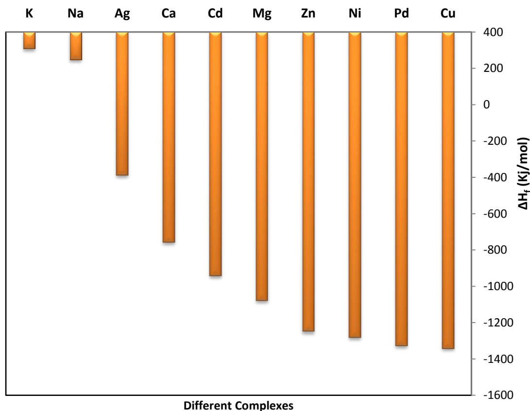
Fig 4. Formation enthalpy changes values for the complexation reaction between 10 cations and 6,15-diazabenz[a][1,4]benzothiazino[3,2-c]phenothiazine.
