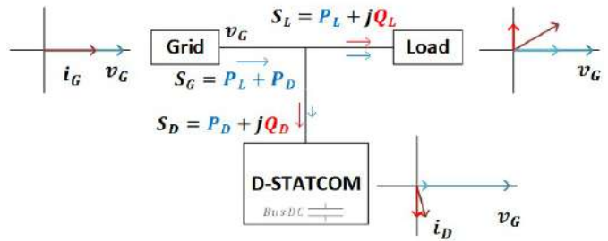
Figure 5. D-STATCOM compensation. Source: own.
