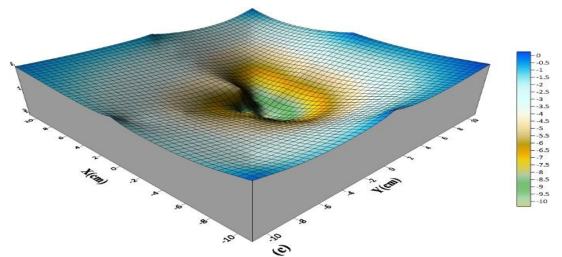
Fig. 7(c): The Scour and Deposition Pattern around Pier (P 1 ) at angle 0° and flowrate 18L/Sec. The green area denotes maximum pattern.
