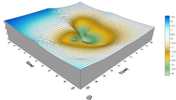
Fig. 7(j): The Scour and Deposition Pattern around Pier ( P_1 ) at angle 15^\circ and flowrate 9 L/Sec.
