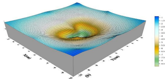
Fig. 7(b): The Scour and Deposition Pattern around Pier (P 1 ) at angle 0° and flowrate 14L/Sec.
