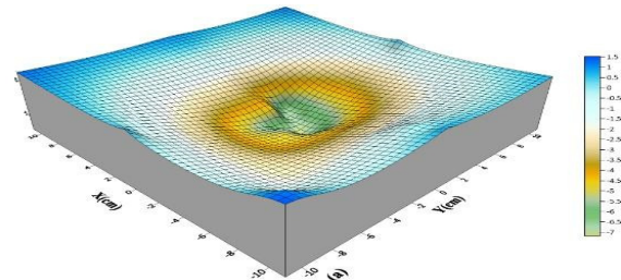
Fig. 7(a): The Scour and Deposition Pattern around Pier (P 1 ) at angle 0° and flowrate 9L/Sec.
