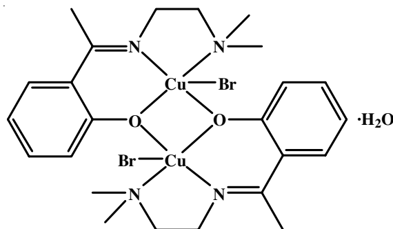
Fig. 5. Structure of \text{Cu}(\text{BrHAP})_2 Schiff base
