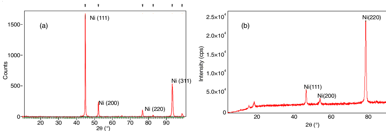
Fig. 5. XRD patterns obtained for nickel electrodeposition from watts bath (a) and optimized bath (b)
