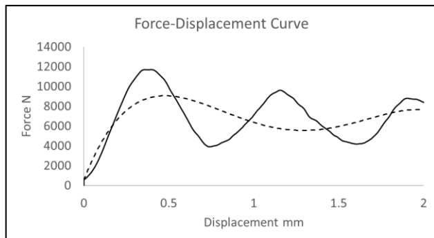
Fig.5. dynamic test results from the impact pendulum tester
