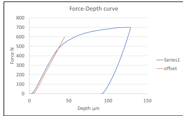
Fig.3. Force-depth curve from indentation test
