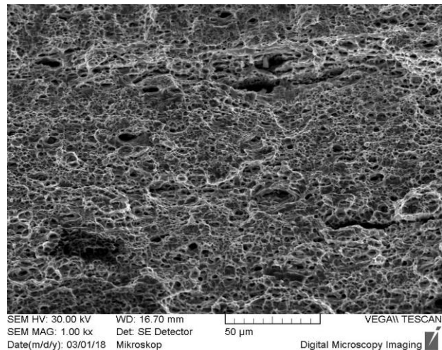
Fig.7. SEM image of the fractured surface after dynamic test
