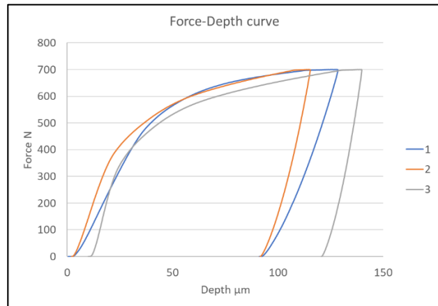
Fig.10. Force-depth curve for the static sample from the fractured end
