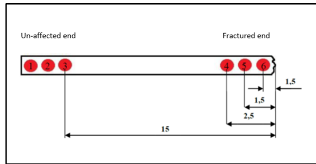
Fig.9. Yield strength measurement positions using indentation technique [14]
