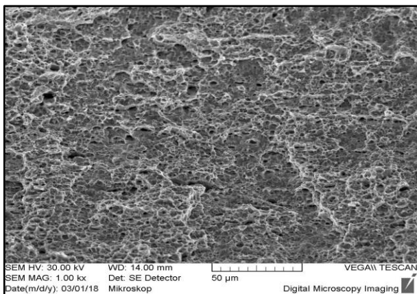
Fig.6. SEM image of the fractured surface after static test
