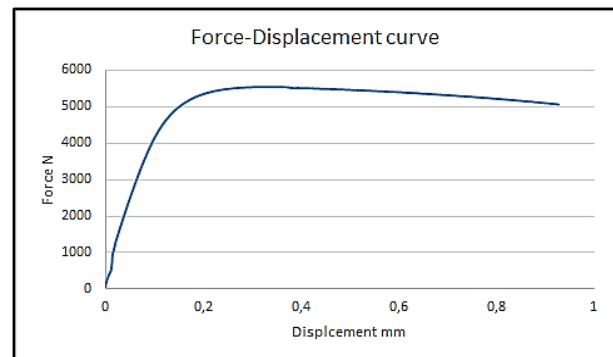
Fig.4. Force-displacement graph for the static tensile test
