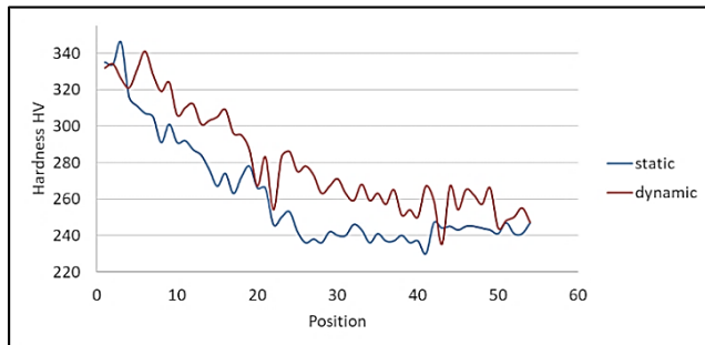
Fig.8. Hardness distribution from fractured end to unaffected end
