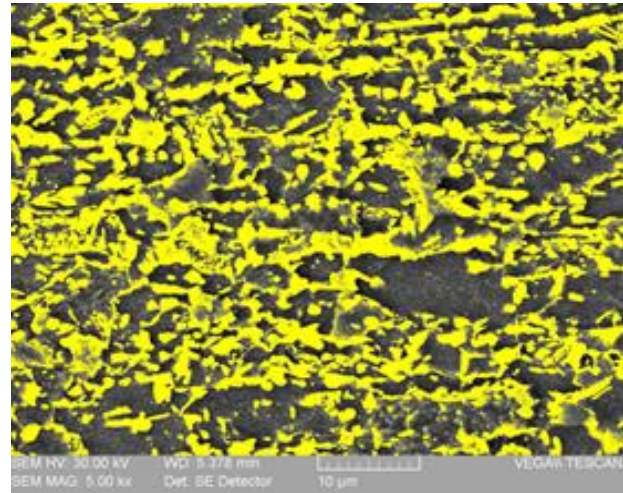
Fig.1. Dual phase steel SEM image
