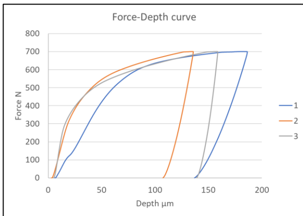
Fig.11. Force -Depth curve for the dynamic sample from the fractured end
