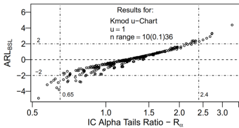
Figure 14. Example of typical ARL_{BSL} vs R_\alpha behaviour for the Kmod u-Chart
