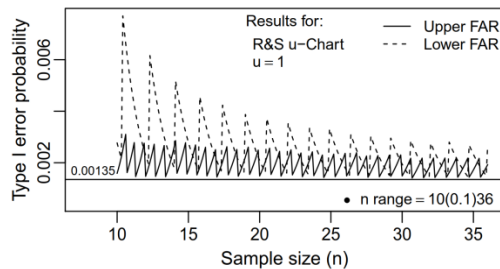
Figure 5. R&S u-Chart upper and lower FARs for u = 1
