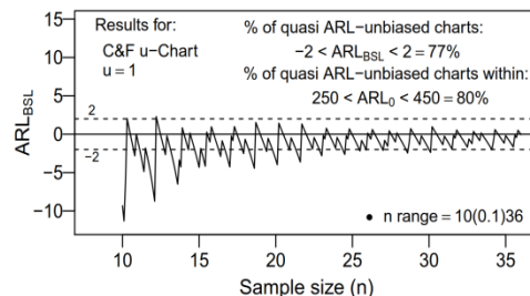
Figure 8. R&S u-Chart ARL_{BSL} values for u=1
