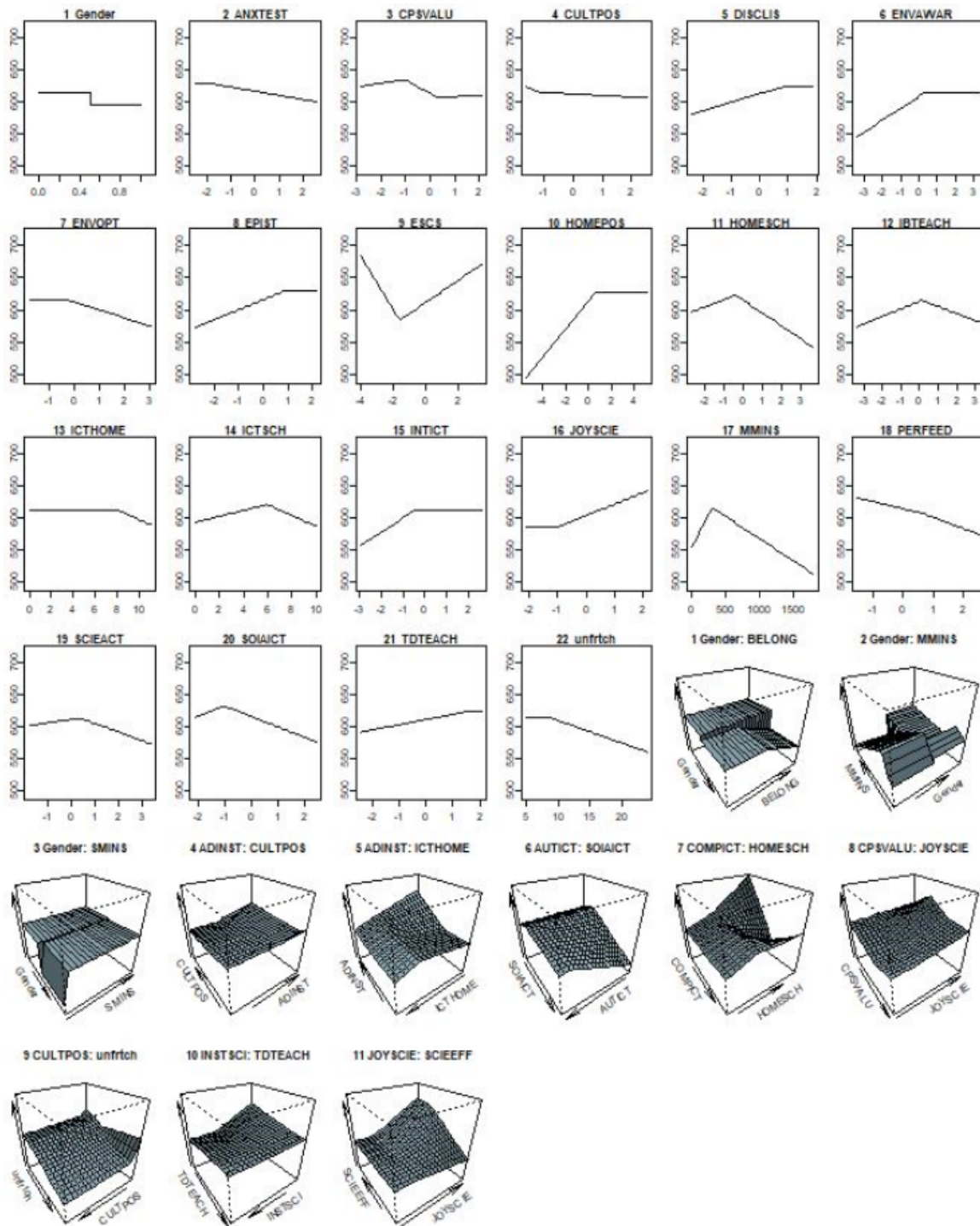
Figure 6. The cutoff points of the variables in the MARS model for the Singapore dataset.
