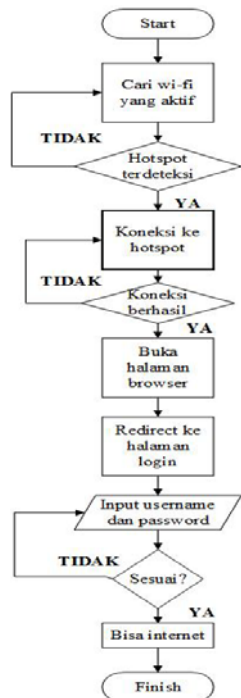
Gambar 2. Flowchart Layanan Hotspot Sistem Single Sign-On.
