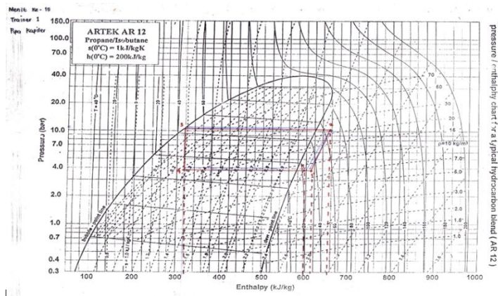
Figure 3: Operating Area of Refrigerant Hydrocarbone (AR12), at Temperature 15 °C
