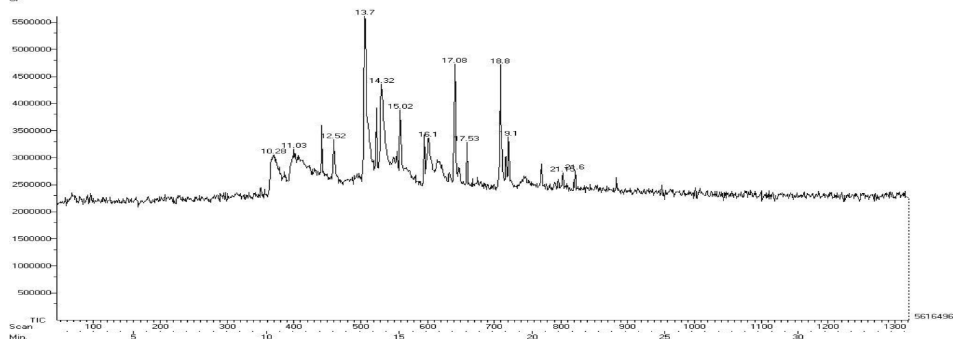
Fig. 1: GC-MS Chromatogram of Chloroform leaf extract of Caesalpinia pulcherrima
