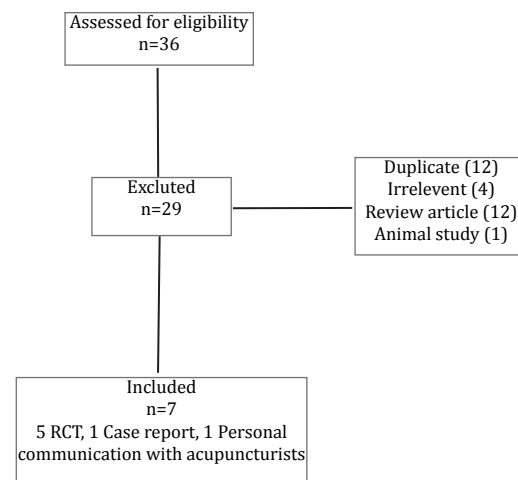
Figure 1. Flowchart study.
