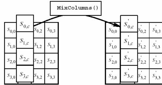
Fig. 4: MixColumns() operates on the State column-by-column.
