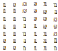
Fig.1: AES algorithm
