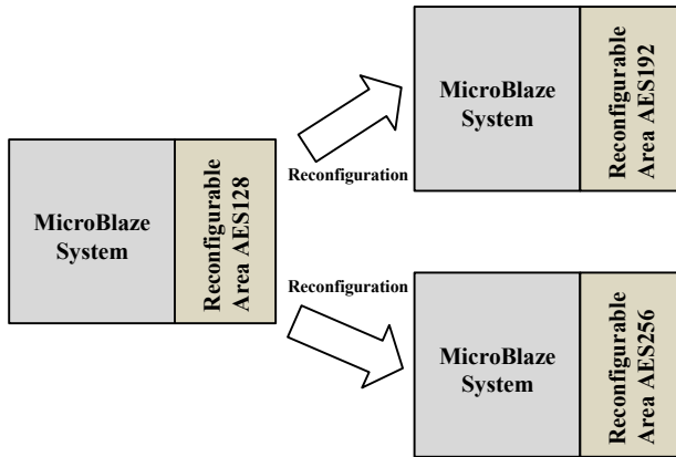
Fig. 10: Modular Design and Reconfiguration cryptosystem.
