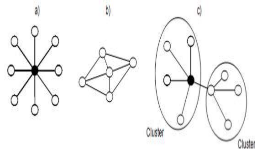
WSN topologies. Star (a), mesh (b), and hybrid
