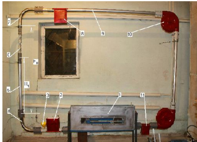
Fig. 8 - Pilot plant
