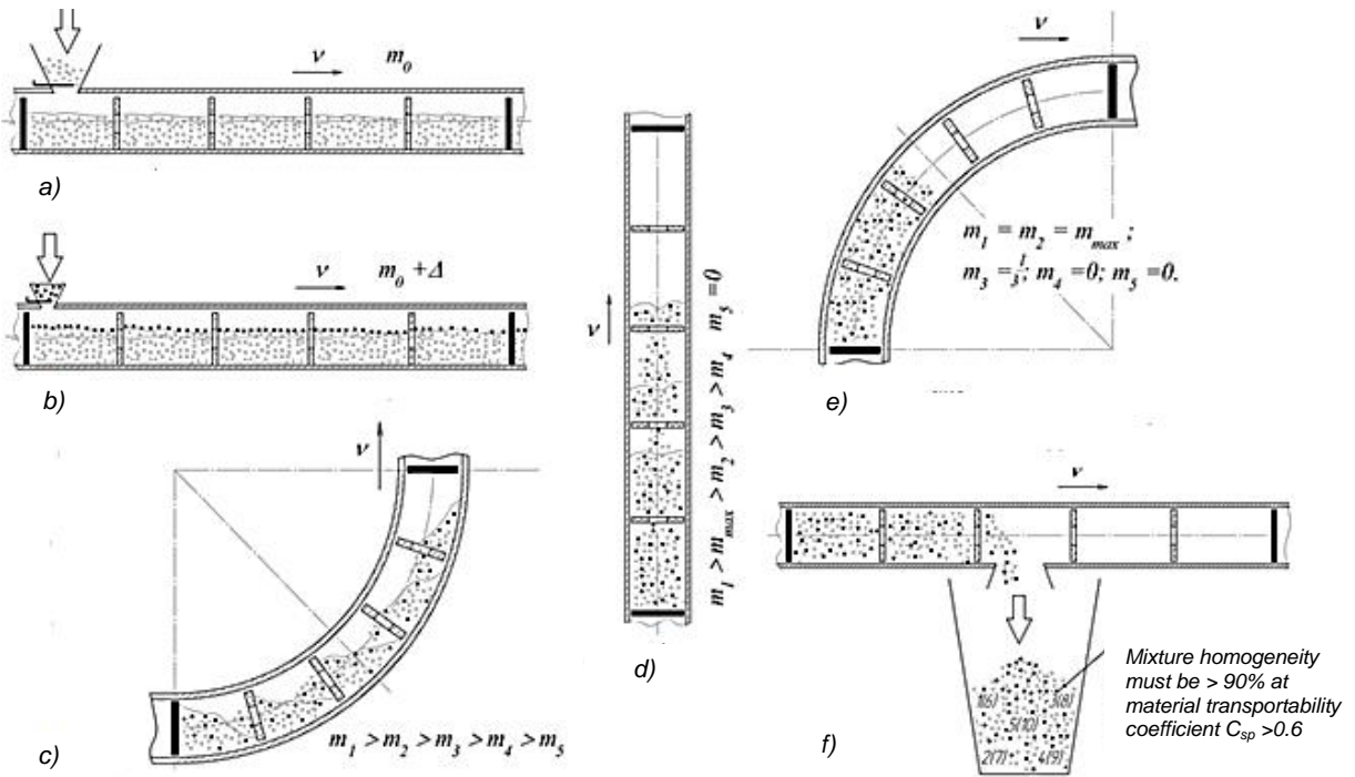
Fig. 1 - Flow sheets of simultaneous transporting and stirring of mixture components - stage – feed of the main component; b – stage – feed of the second component; c – stage – partial stirring of components; d – V stage – main stirring of components; e – V stage – transportation of components; f – V stage – unloading with entire stirring of components
