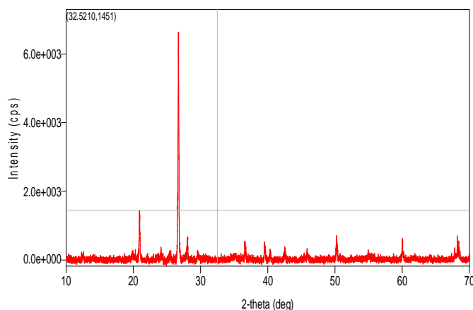
Fig 4 XRD analysis of the Virgin Soil
