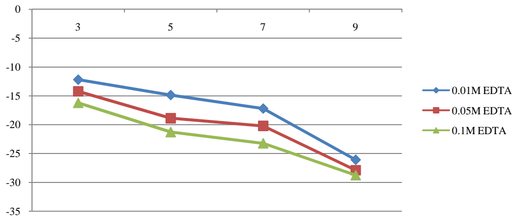
Fig.7 Zeta Potential of decontaminated soil at different EDTA concentration
