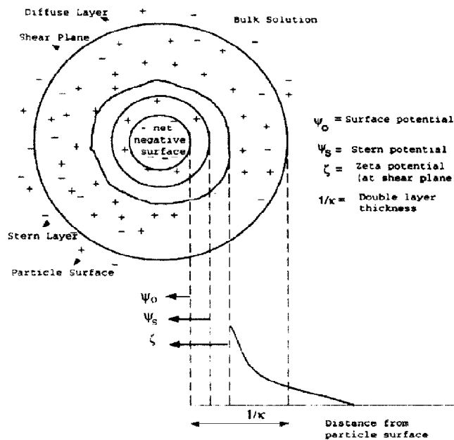
Fig.1 The location of zeta potential, \zeta , on the electrical diffuse double layer (Yukselen et al [8])
