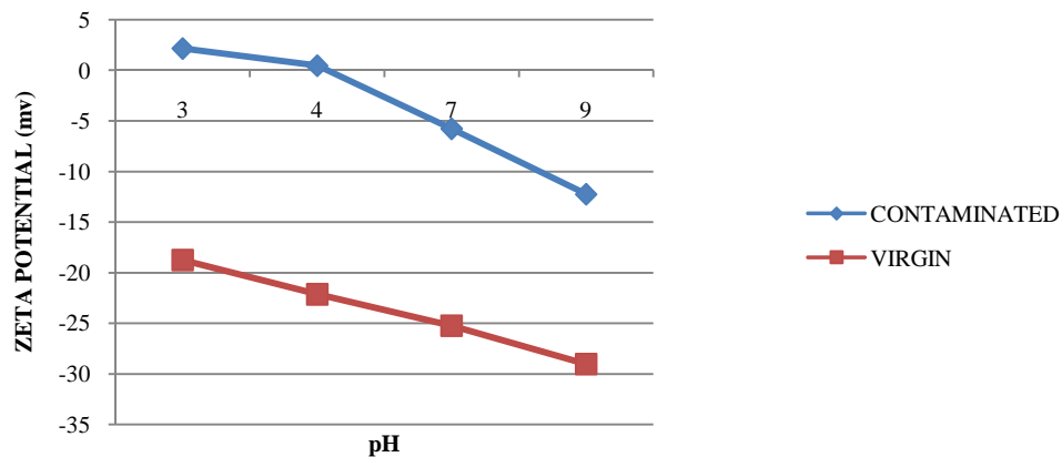
Fig.6 Comparative study of Zeta potential of Virgin and Contaminated Soil
