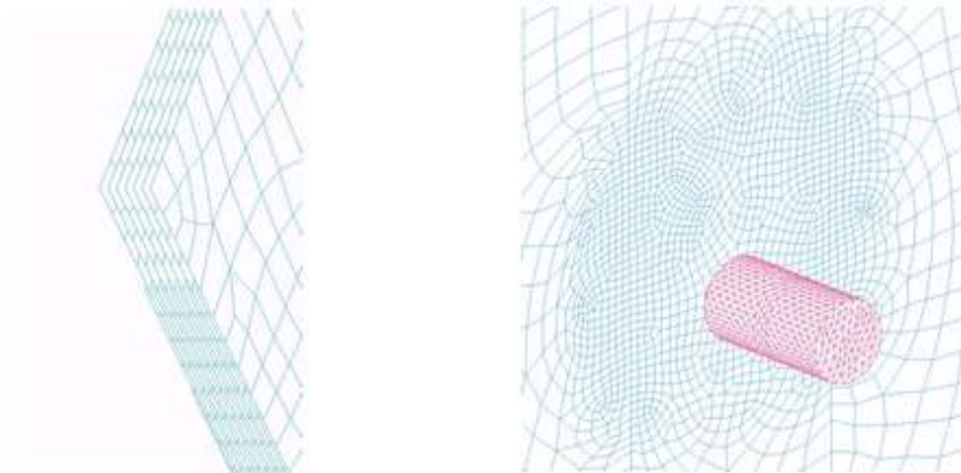
Figure 11. Details of discretisation: layers and impact zone
