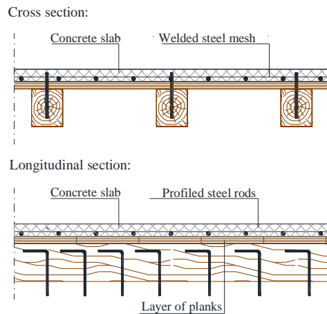
Figure 13. Transverse and longitudinal sections of a typical intervention of floor reinforcement with RC slab and steel connectors
