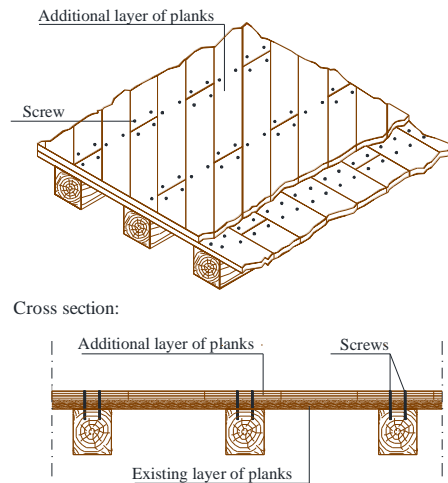
Figure 14. Floor reinforcement with additional layers of planks.
