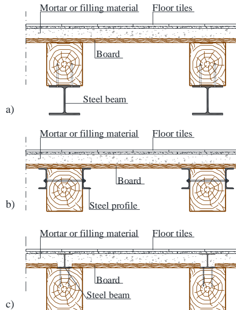
Figure 16. Steel profile reinforcements at a, b) intrados or c) extrados of wooden beams
