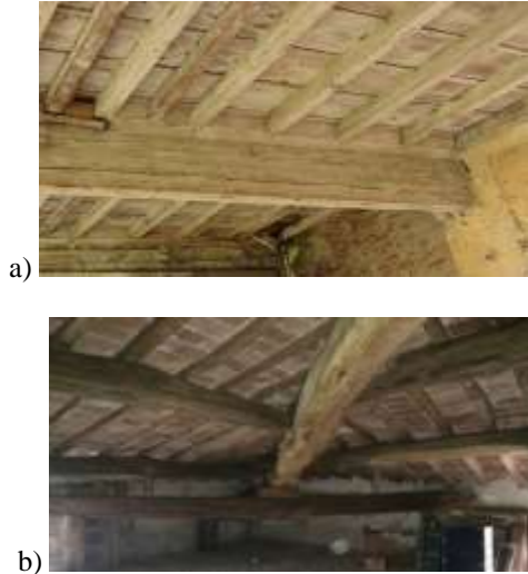
Figure 12. Common floor or pitch structural typologies: (a) wood planks nailed to the underlying rafters; (b) a layer of thin solid bricks resting on the rafters.
