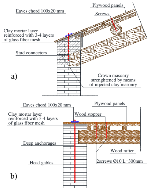
Figure 31. Wood diaphragm – masonry connection: a) transverse section on longitudinal masonry wall, b) transverse section on head gables
