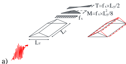
Figure 10. Roof subject to earthquake action in the transverse direction: scheme of forces acting on roof pitches and lateral gables.
