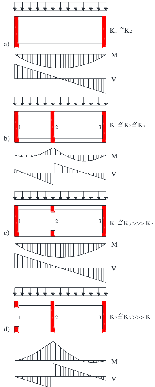
Figure 8. Examples of in-plane bending and shear diagrams for the floor diaphragm: (a) isostatic and (b-d) hyperstatic WRS configurations
