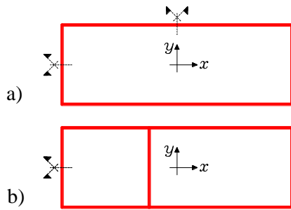
Figure 7. Examples of (a) isostatic and (b) hyperstatic WRS configurations in a masonry building
