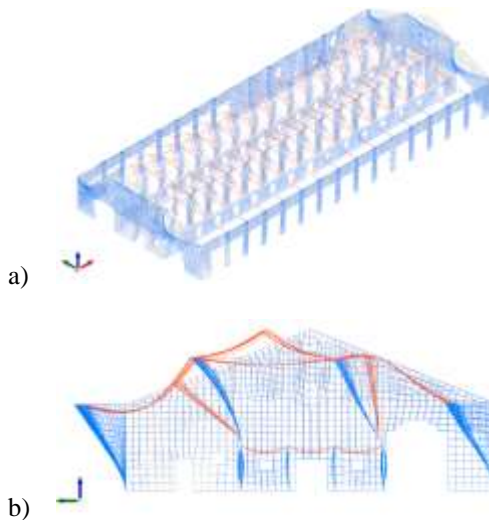
Figure 28. FEM modelling of the barn before retrofit - Displacements for earthquake action in the transverse direction: a) global view and b) lateral displacements in a transverse section gable far from the two masonry gable walls.
