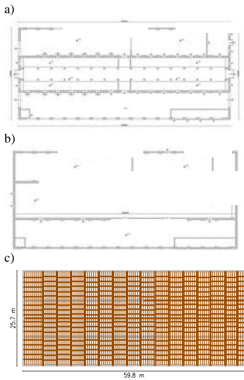
Figure 23. a) ground floor plan, b) first floor plan, c) arrangement of timber roof beams and rafters
