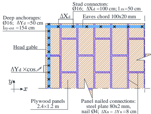
Figure 38. Reinforcement of the barn roof with multi-layered wood panels - Plan view of a portion of the roof
