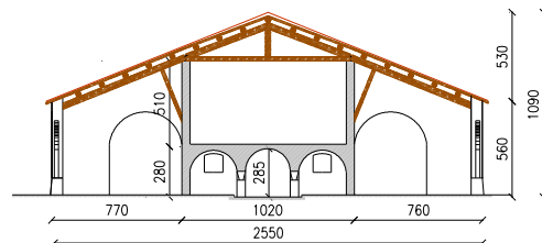
Figure 22. Typical cross-section of the barn with indication of the main wooden structure
