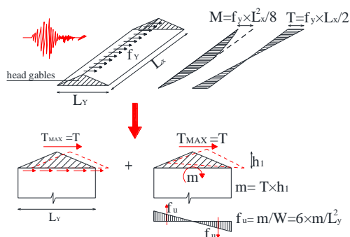
Figure 10. Roof subject to earthquake action in the transverse direction: scheme of forces acting on roof pitches and lateral gables.
