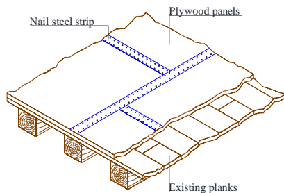
Figure 15. Floor reinforcement with multi-layered wood panels.
