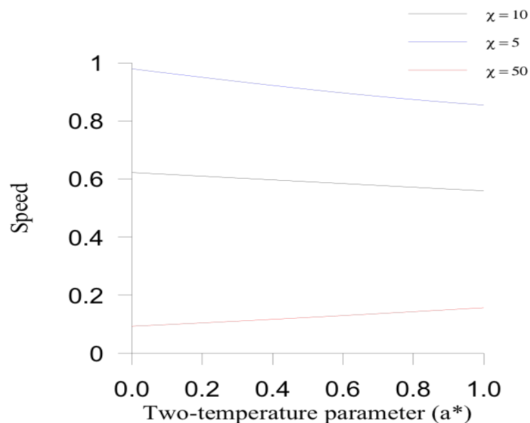
Figure 3. Variation of non-dimensional speed ( c^2/c_2^2 ) against two-temperature parameter a^* , when \chi = 5, 10, 50 .
