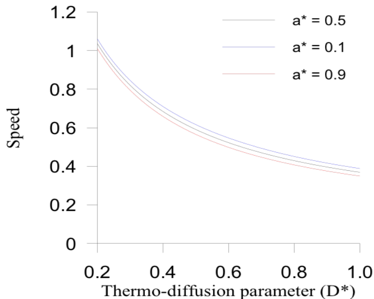
Figure 1. Variation of non-dimensional speed ( c^2/c_2^2 ) against thermodiffusion parameter D^* , when a^* = 0.1, 0.5 and 0.9 .
