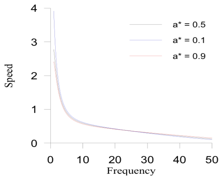
Figure 2. Variation of non-dimensional speed ( c^2/c_2^2 ) against frequency \chi , when a^* = 0.1, 0.5 and 0.9 .
