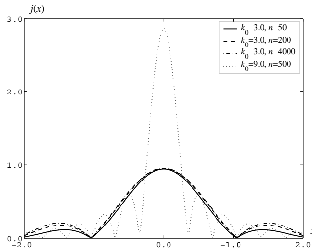
Fig. 4. The currents j(x) for several parameters k_0 , h(k) = 1 .
