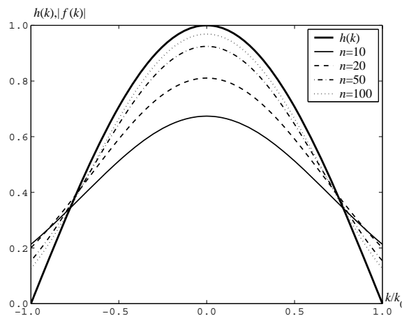
Fig. 1. The given h(k) = \cos(\pi k / 2k_0) and the obtained f(k) diagrams.
