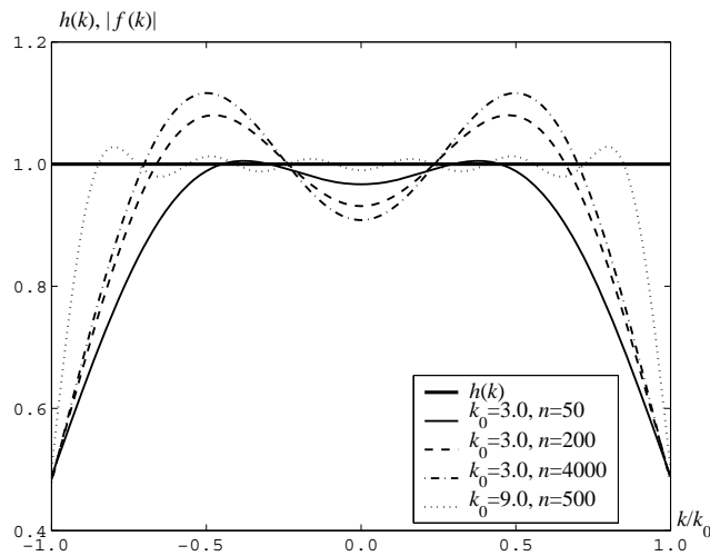
Fig. 3. The given h(k) = 1 and the obtained |f(k)| diagrams.
