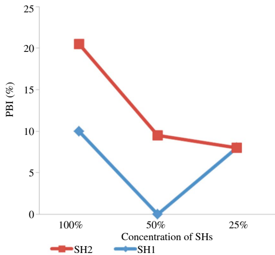
Figure 1. Growth inhibitory activity of the SHs against S. aureus .
