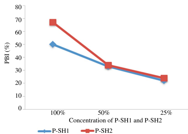
Figure 6. Growth inhibitory activity of the P-SHs against E. coli .
