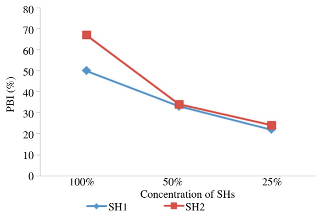
Figure 3. Growth inhibitory activity of the SHs against E. coli .
