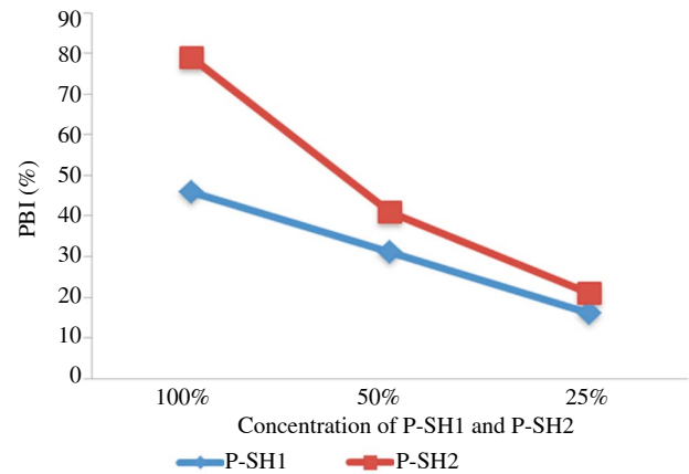
Figure 4. Growth inhibitory activity of the P-SHs against S. aureus .
