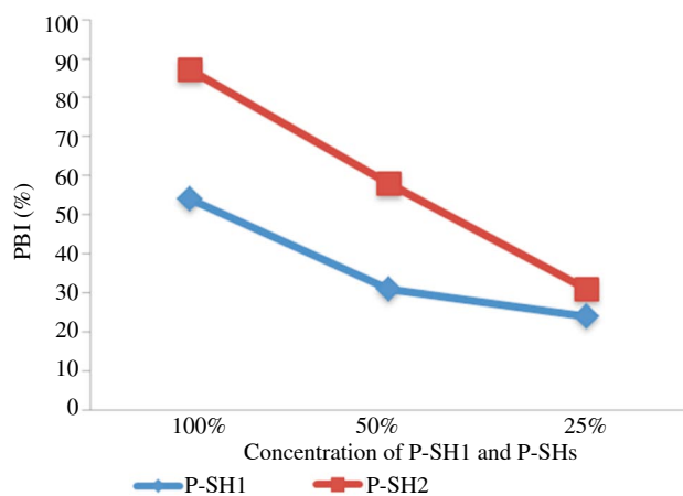
Figure 5. Growth inhibitory activity of the P-SHs against P. aeruginosa .
