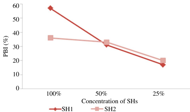
Figure 2. Growth inhibitory activity of the SHs against P. aeruginosa .
