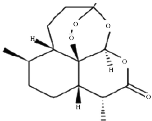
Figure 2. Artemisinin.
