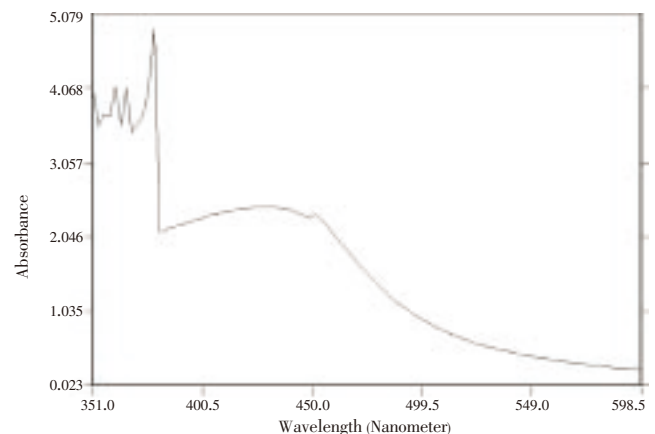
Figure 1. UV-VIS absorption spectra of Ag nanoparticle synthesized from M. oleifera leaves extract at 1 mM silver nitrate.
