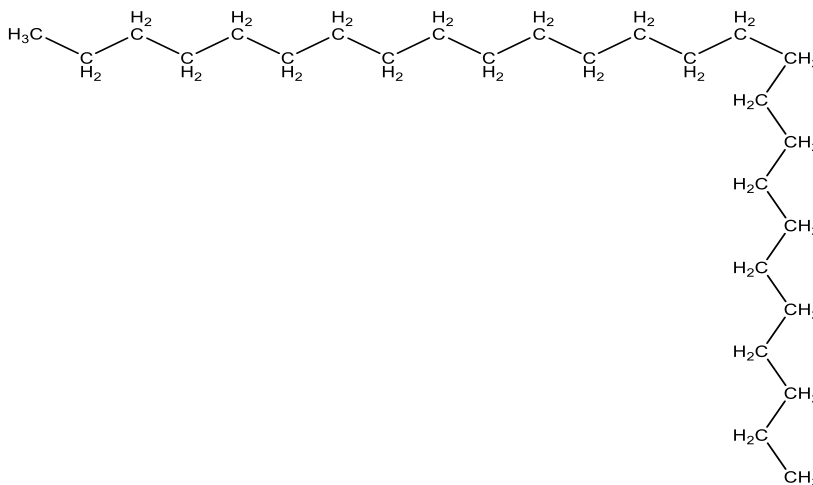
Figure 3. Hexacosane.
