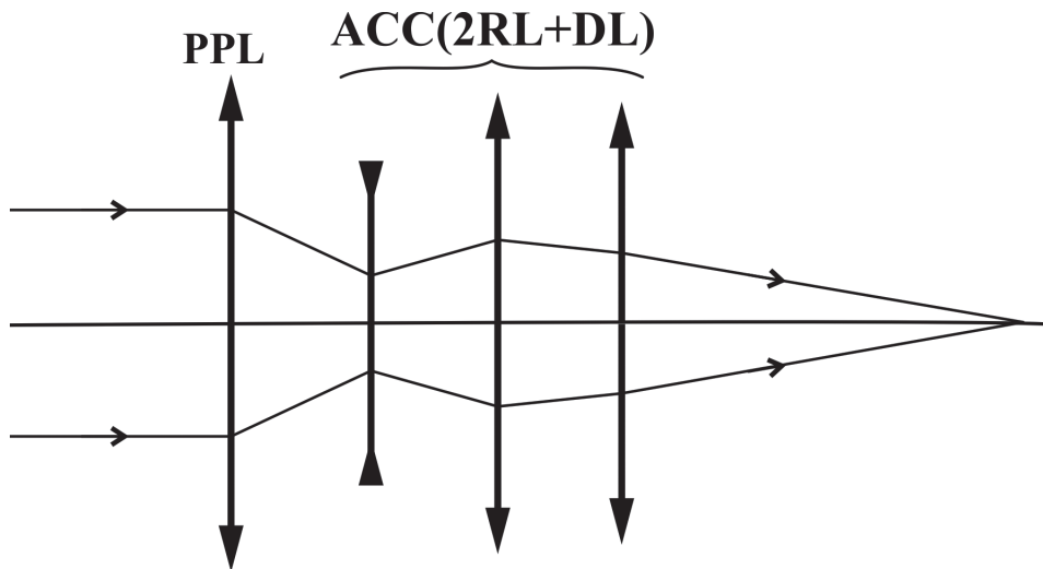
Fig. 1. Optical scheme of the model achromatic objective, whose ACC consists of two RL and DL, and PPL is made of PMMA and has normalized optical force equal to 0.50 (see. Table 1). Normalized optical forces of two RL and DL are respectively -0.27; 0.76; 0.01
