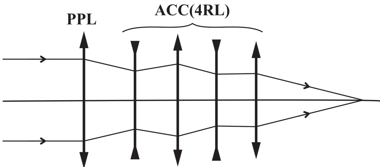
Fig. 2. Optical scheme of model objective- superachromate, whose ACC consists of four RL, and PPL is made of POLYCARB and has a normalized optical power equal to 0.80 (see. Table. 2). The normalized optical power of four RL are respectively -1.08; 1.07; -0.39; 0.60
